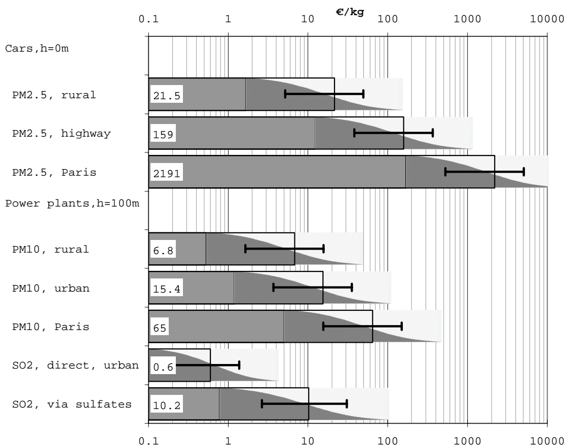
Figure 2. Typical damage costs for PM and SO 2 (values of ExterneE 1998 for France), together with the uncertainty range. The gray curve indicates the probability that the true cost is below a specified value. The mean damage costs are shown in the labels. On a log plot the distribution is symmetric about the median which is lower than the mean. The error bars indicate 1 geometric standard deviation (68% confidence interval).
